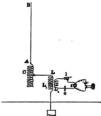
FIG. 63.—Particular Set of Tuned Receiving Connections.
